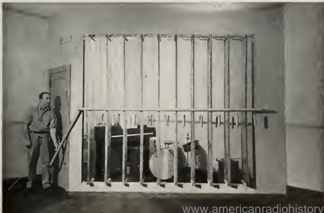
ACOUSTICAL FILTERS USED IN RADIO-MUSIC TEST.
